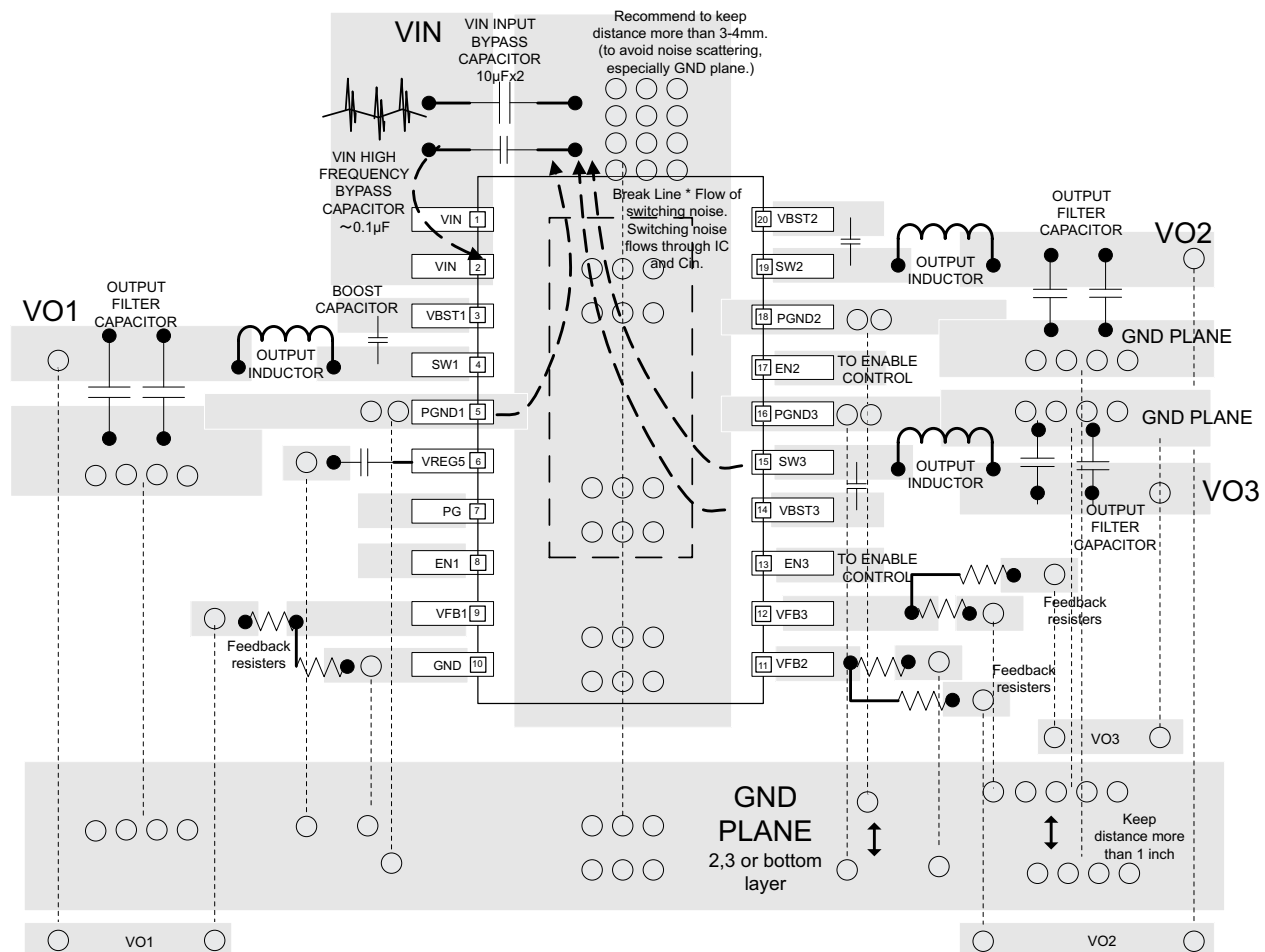
Figure 37. TPS65580 Layout
