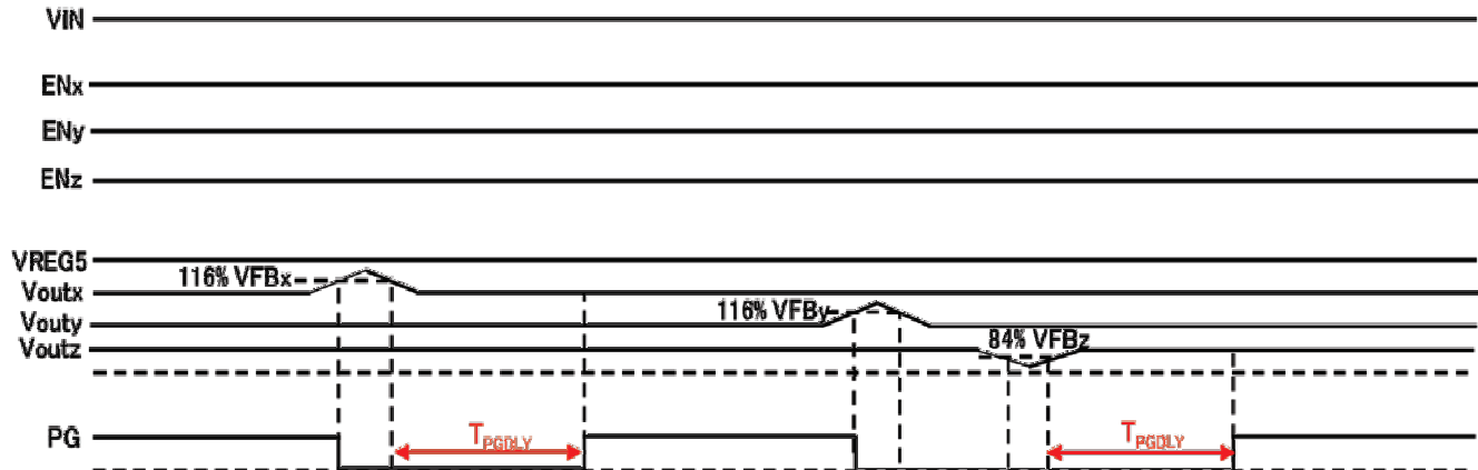
Figure 2. V_{OUT} Transient
