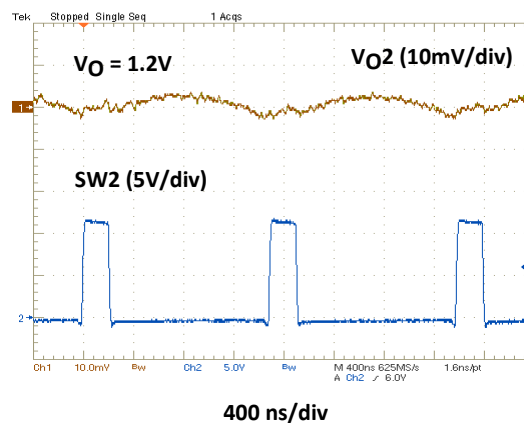
Figure 27. VOUT2 = 1.2V, Ripple Voltage at IOUT2 = 2.5A
