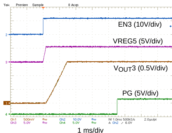
Figure 34. VOUT3 = 1.5V Soft-Start IOUT3 = 1.5A
