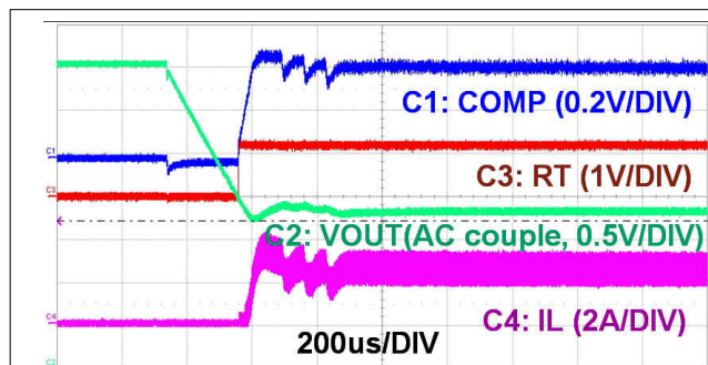
Figure 9-4. Automatic Wake-Up
