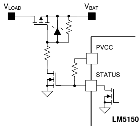
Figure 9-2. Disconnection Switch Control Example
