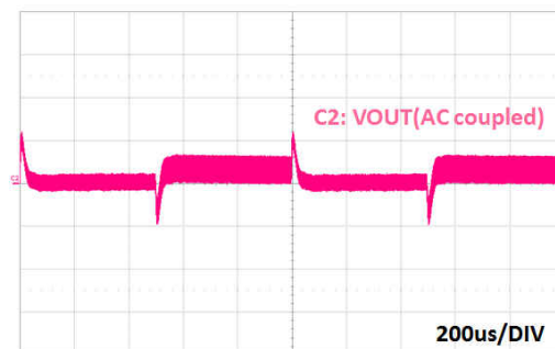
Figure 9-5. Load Transient (3 A to 1.5 A, 0.1 V/DIV)
