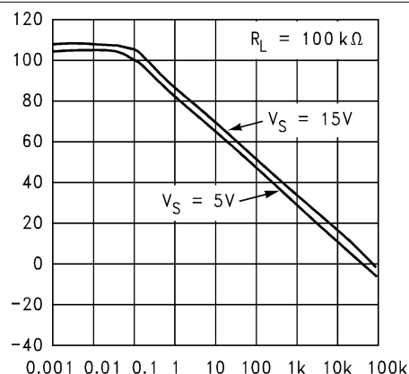
Figure 6-12. Open-Loop Frequency Response
