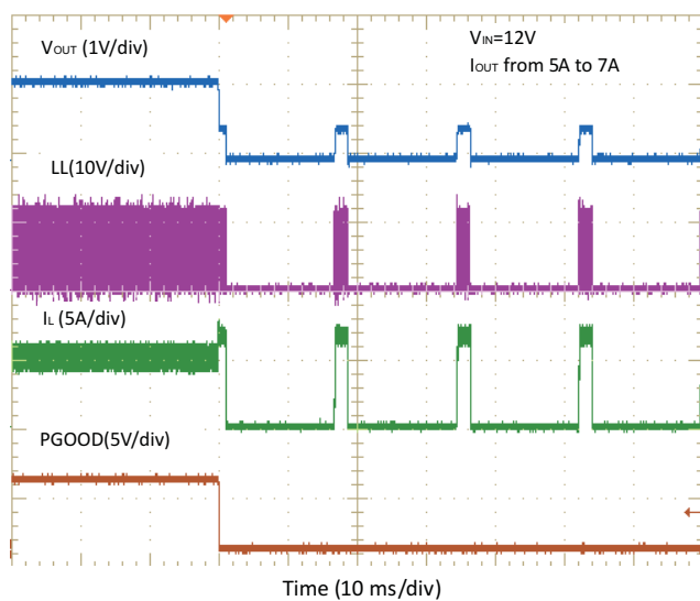
Figure 29. Overcurrent Protection
