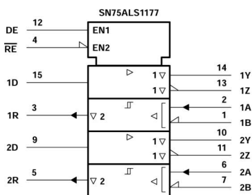
Logic Symbol†
