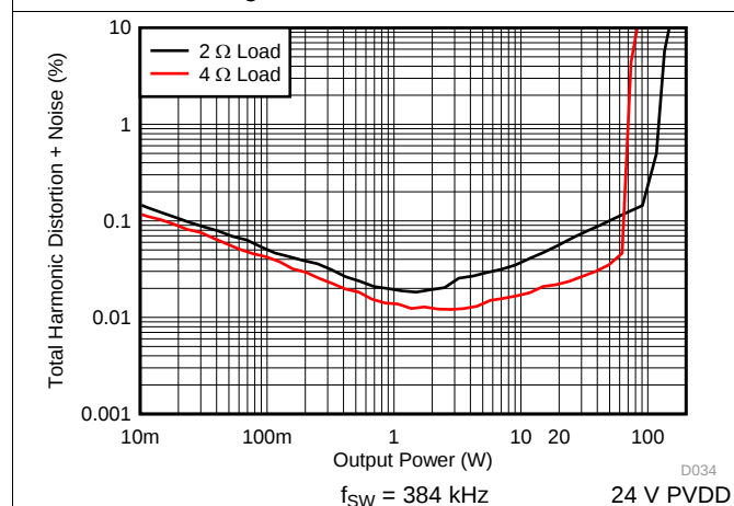
Figure 29. PBTL THD+N vs Power
