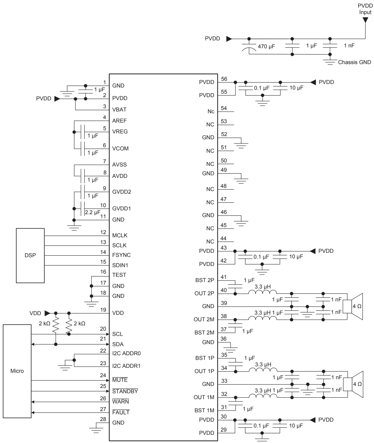
Figure 77. Typical 2-Channel BTL Application Schematic
