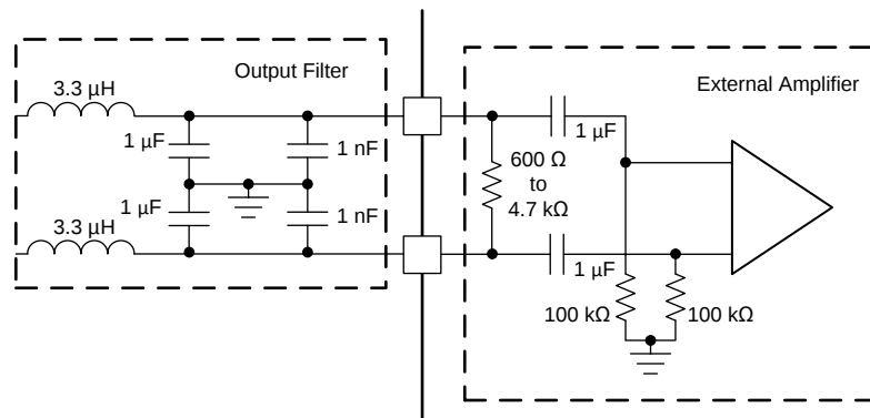
Figure 76. External Amplifier Input Configuration for Line Driver
