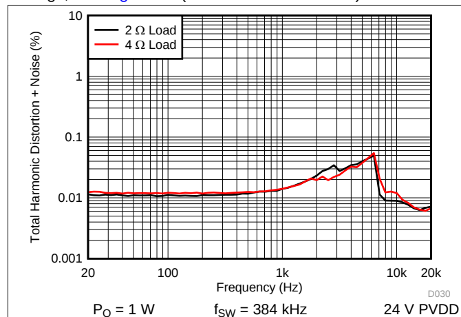
Figure 25. PBTL THD+N vs Frequency
