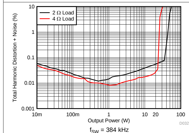
Figure 27. PBTL THD+N vs Power
