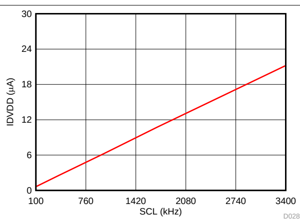
Figure 70. I_{DVDD} in Manual Mode with SCL
