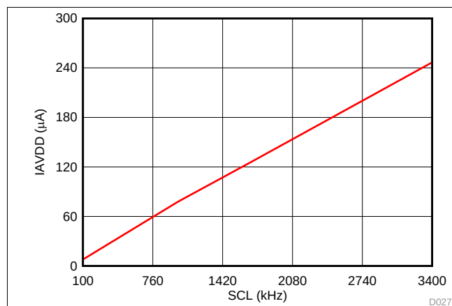
Figure 69. I_{AVDD} in Manual Mode with SCL
