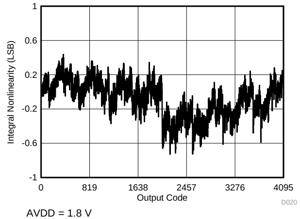
Figure 20. Typical INL in Manual Mode
