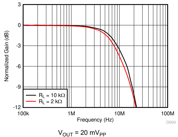
Figure 7-6. Small-Signal Frequency Response vs Output Load Load
