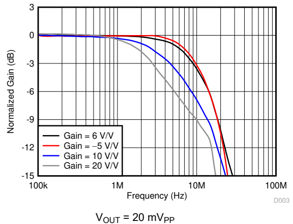
Figure 7-4. Small-Signal Frequency Response vs Gain
