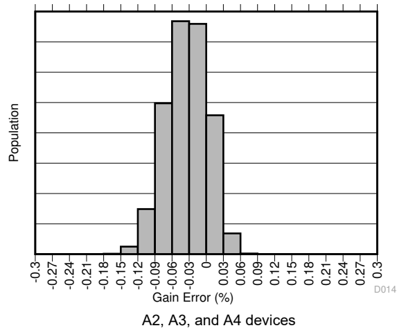
Figure 6-6. Gain Error Production Distribution
