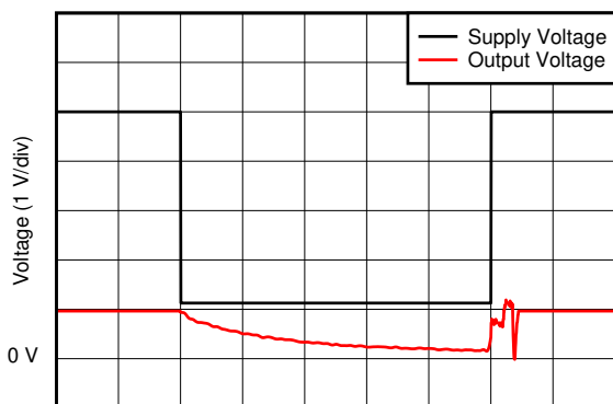
Figure 6-25. Noninverting Differential Input Overload
