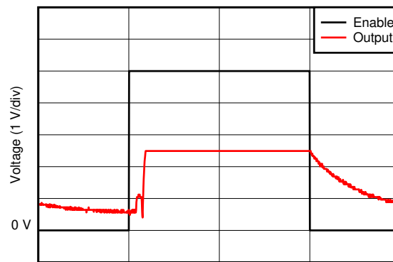
Figure 6-26. Start-Up Response
