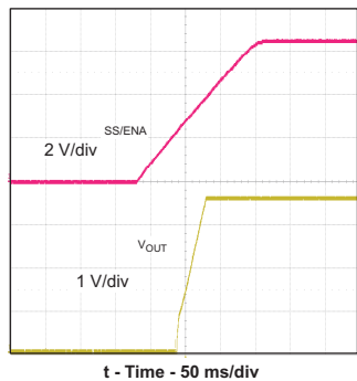
Figure 17. Slow-Start Timing
