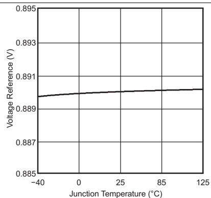
Figure 5. Voltage Reference vs Junction Temperature
