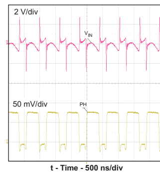
Figure 18. Input Ripple
