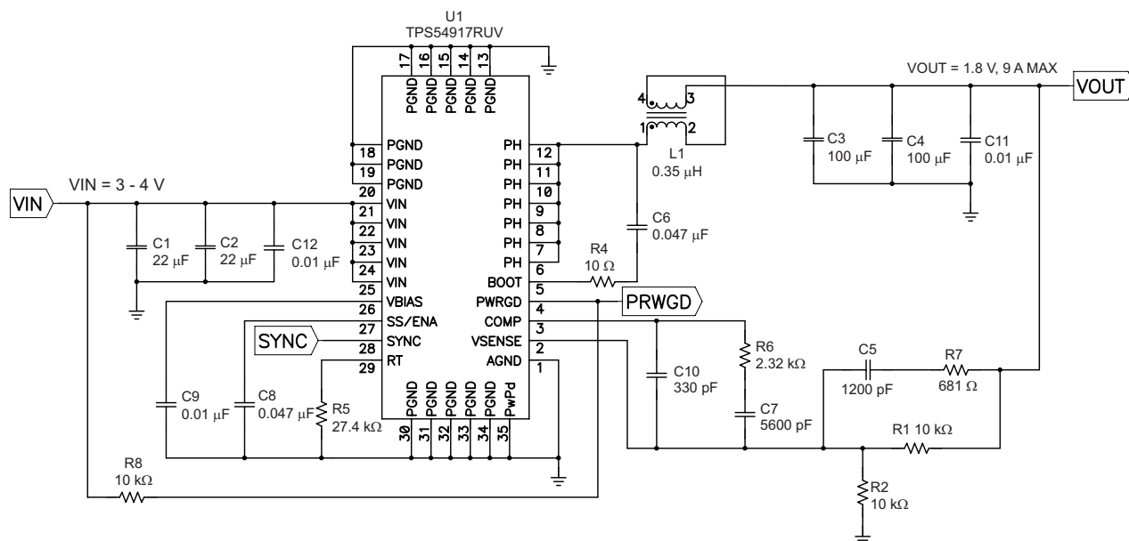
Figure 10. Application Circuit
