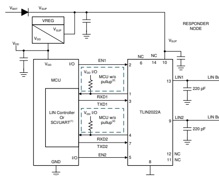
Simplified Schematics, Responder Mode
