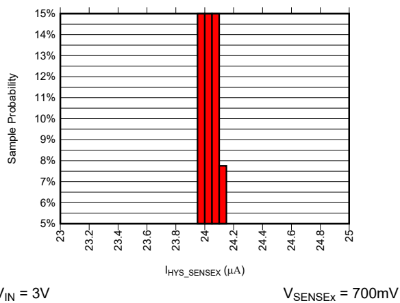
Figure 6-9. I_{HYS\_SENSEX} Current Distribution at Temperature of 125^{\circ}C
