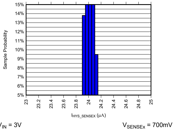
Figure 6-7. I_{HYS\_SENSEX} Current Distribution at Temperature of -55^{\circ}C
