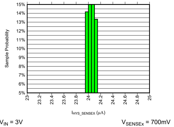
Figure 6-8. I_{HYS\_SENSEX} Current Distribution at Temperature of 25^{\circ}C
