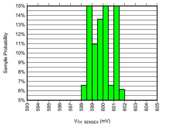
Figure 6-11. V_{TH\_SENSEX} Voltage Distribution at Temperature of +25^{\circ}C
