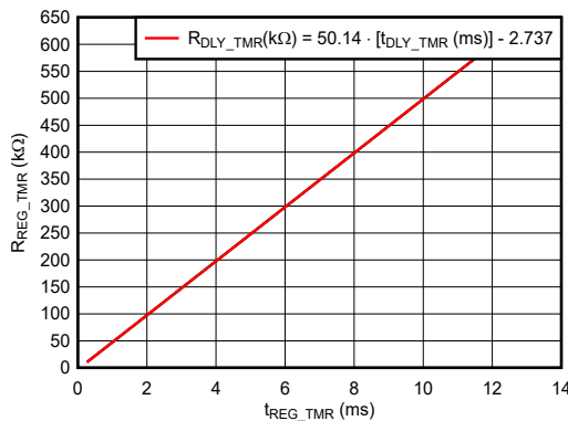
Figure 8-11. R_{REG\_TMR} vs t_{REG\_TMR} From 0.264ms to 12.4ms
