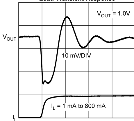
2 \mu\text{s/DIV} Figure 17.
