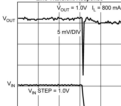
20 \mu\text{s/DIV} Figure 15.
