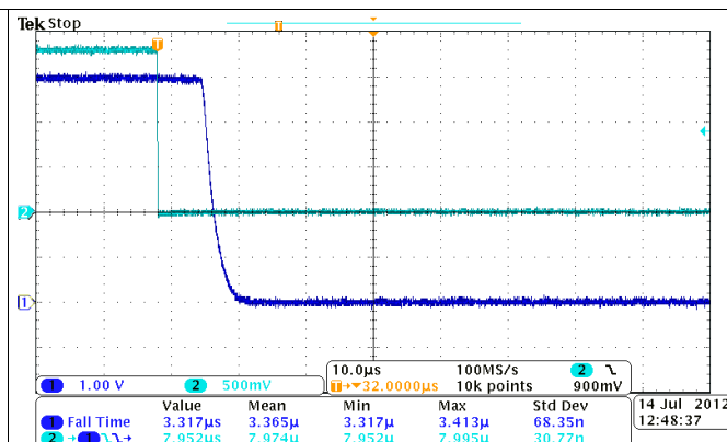
Figure 30. Turnoff Response Time (V_{IN} = 5\text{ V}, V_{BIAS} = 5\text{ V}, C_{IN} = 1\text{ μF}, C_L = 0.1\text{ μF}, R_L = 10\text{ Ω}) CH1: VOUT, CH2: ON
