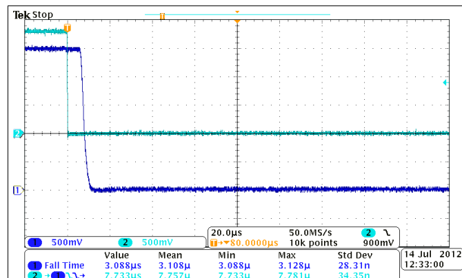
Figure 29. Turnoff Response Time (V_{IN} = 2.5\text{ V}, V_{BIAS} = 2.5\text{ V}, C_{IN} = 1\text{ μF}, C_L = 0.1\text{ μF}, R_L = 10\text{ Ω}) CH1: VOUT, CH2: ON
