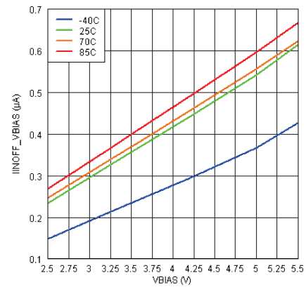
Figure 3. V_{BIAS} vs Shutdown Current
