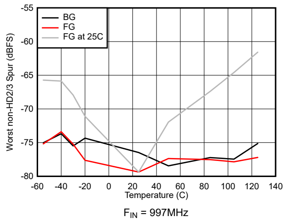
Figure 5-39. Worst non-HD2/3 Spur vs Temperature
