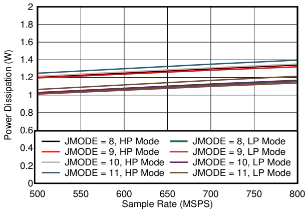
Figure 5-83. Dual Channel, Power Dissipation vs F_S for JMODES 8 - 11
