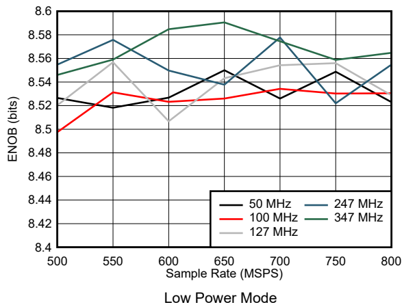
Figure 5-27. ENOB vs Sample Rate
