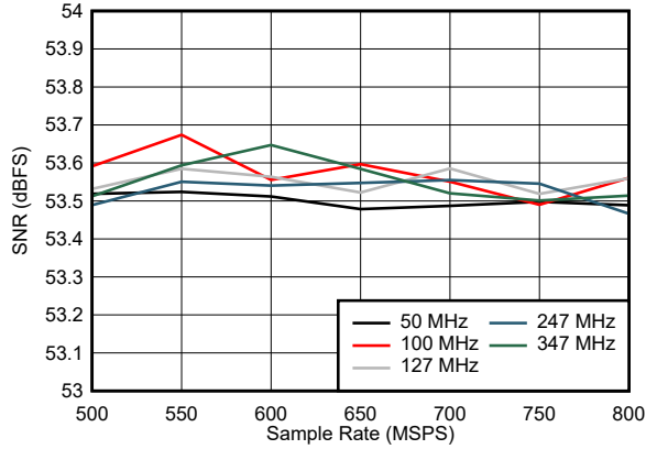
Figure 5-25. SNR vs Sample Rate
