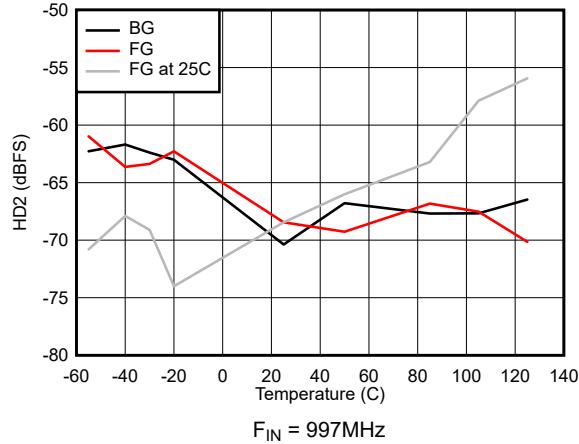
Figure 5-37. HD2 vs Temperature
