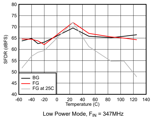
Figure 5-41. SFDR vs Temperature
