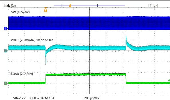
Figure 7-8. Load Transient
