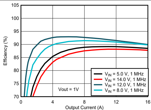
Figure 7-4. Efficiency Curves
