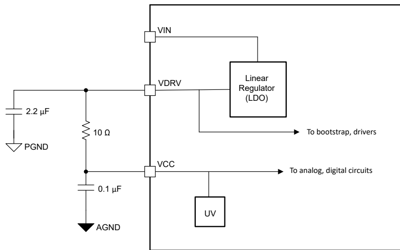
Figure 6-1. Device Bypassing
