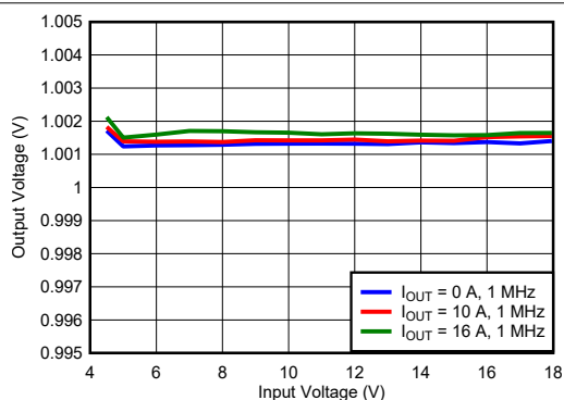
Figure 7-6. Line Regulation
