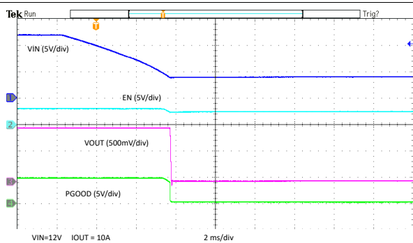
Figure 7-15. V_{IN} Shutdown
