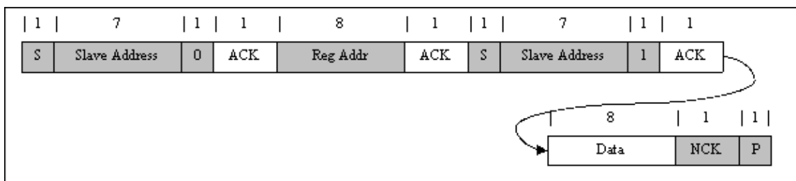
Figure 8-19. Single Read
