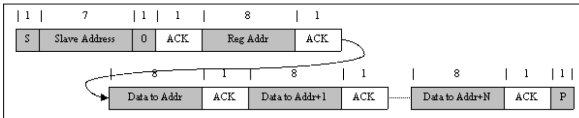
Figure 8-20. Multi-Write
