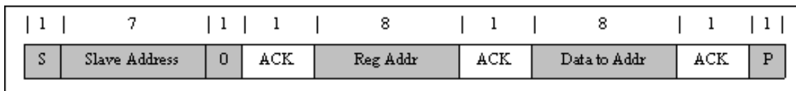
Figure 8-18. Single Write
