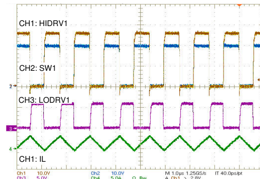
Figure 10-8. PWM Operation
