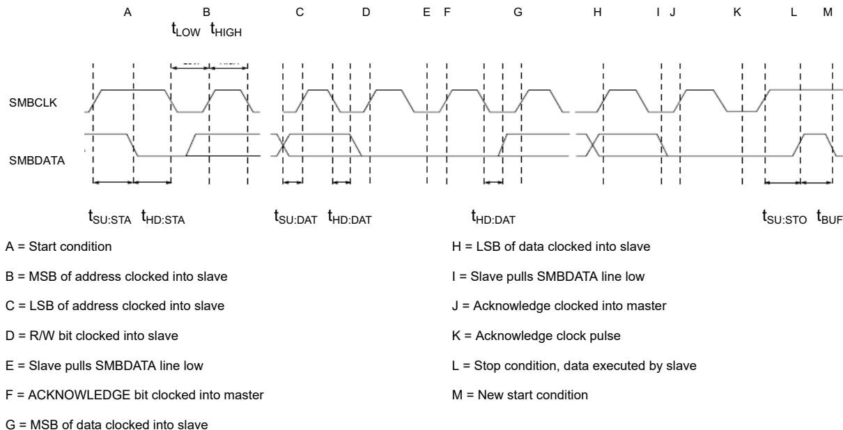
Figure 9-4. SMBus Write Timing
