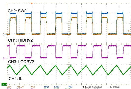
Figure 10-7. PFM Operation
