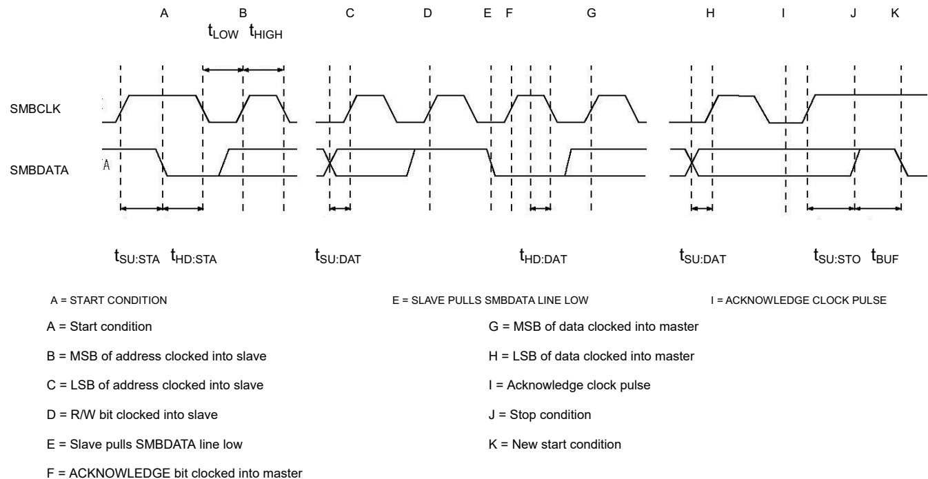
Figure 9-5. SMBus Read Timing
