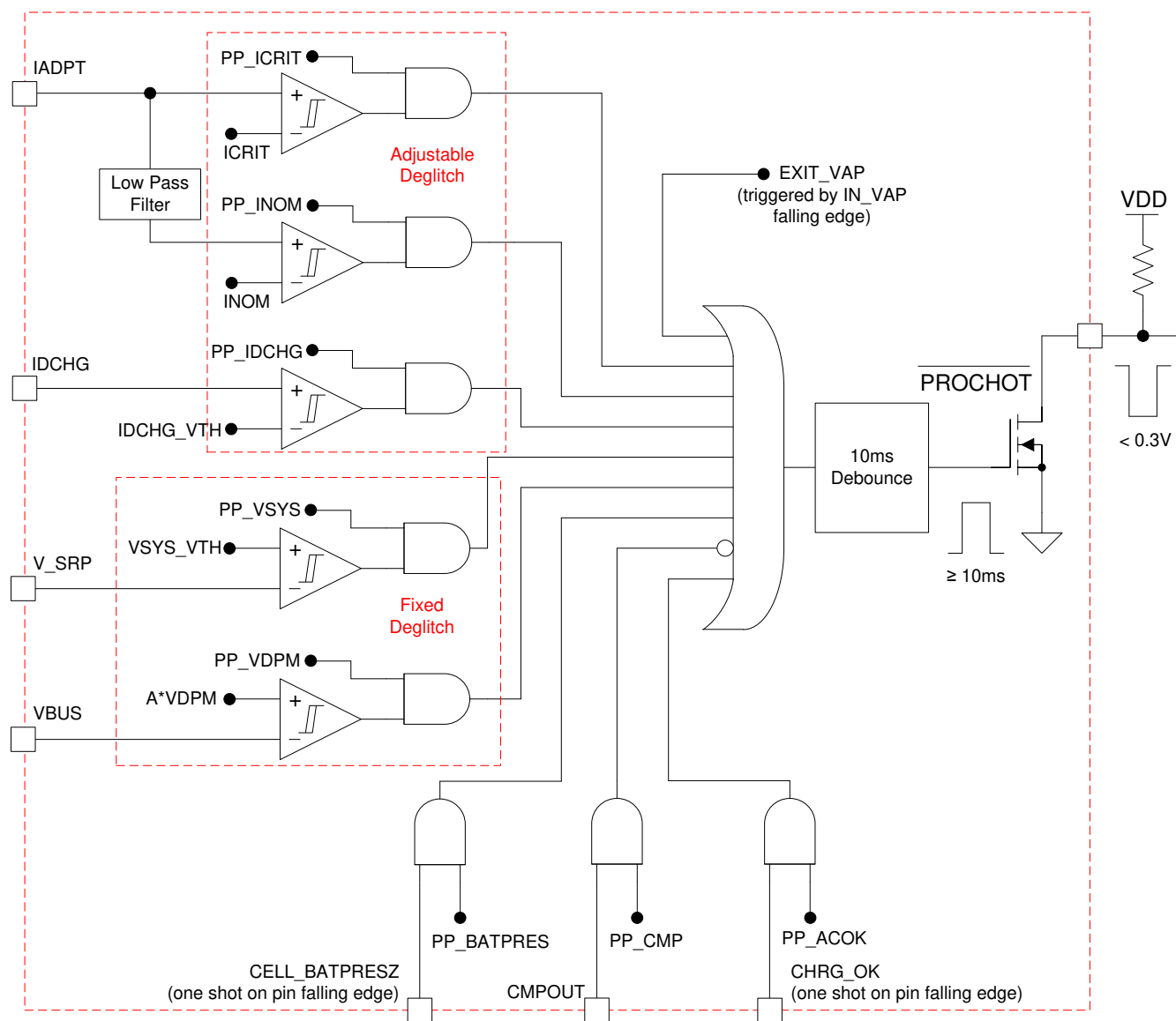
Figure 9-2. PROCHOT Profile
