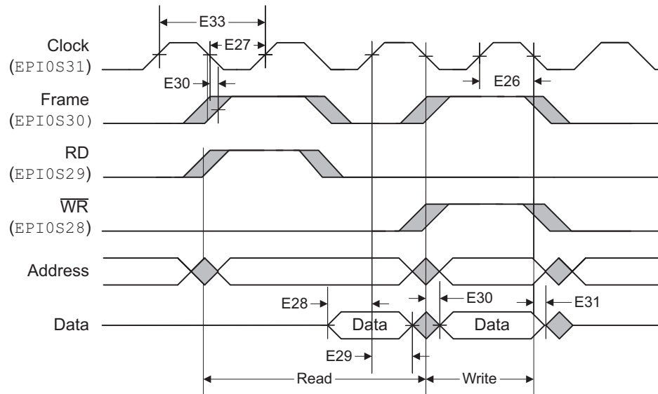
Figure 5-28. General-Purpose Mode Read and Write Timing
