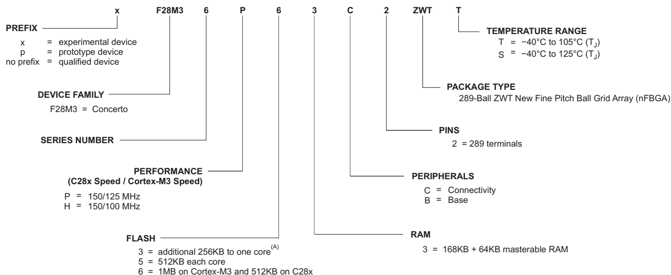
Figure 8-1. Device Nomenclature
