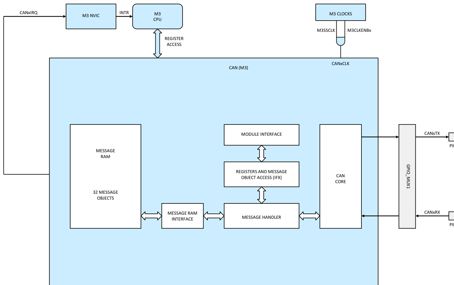
Figure 5-33. CAN (Cortex-M3)
