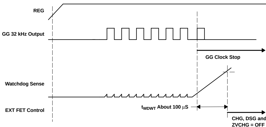
Figure 3. Watchdog Timing Chart—WDI Fault After Startup
