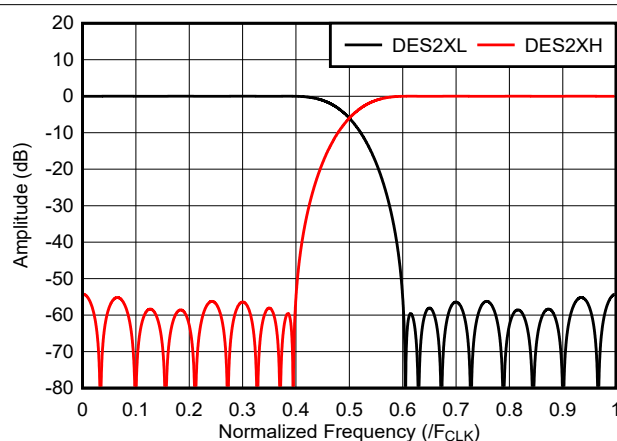
Figure 7-48. DES Interpolator Frequency Response
