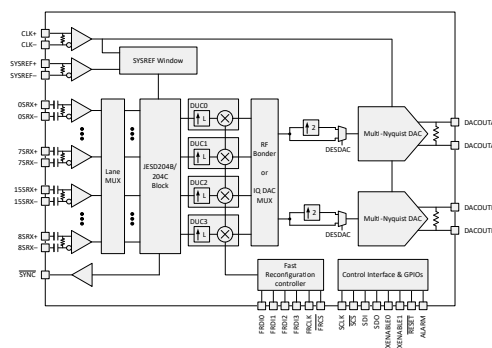
Block Diagram
