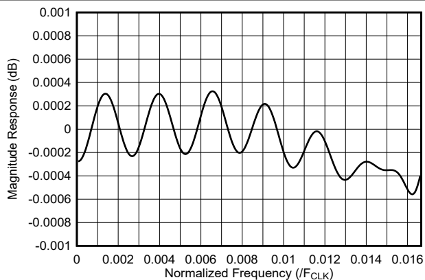
Figure 7-29. 24x Interpolation Filter Passband Response
