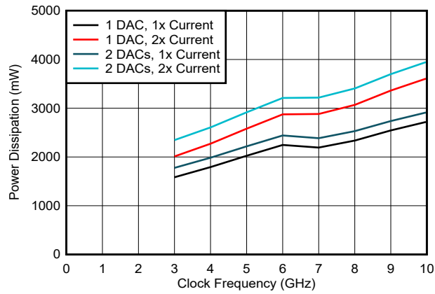
Figure 6-215. Power Dissipation vs Clock Frequency and DAC Mode
