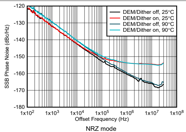
Figure 6-204. Phase Noise vs Offset Frequency at 1 GHz
