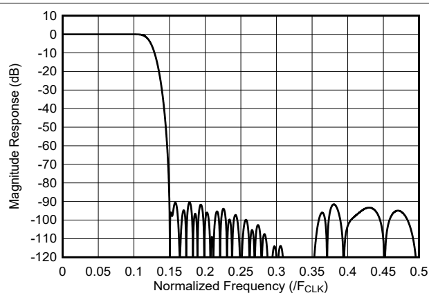
Figure 7-18. 4x Interpolation Filter Response
