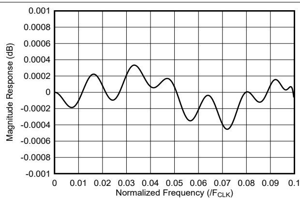
Figure 7-19. 4x Interpolation Filter Passband Response
