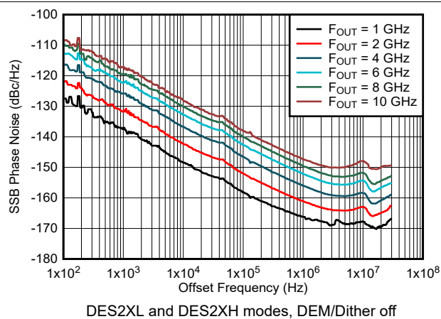
Figure 6-203. Phase Noise vs Offset Frequency and Output Frequency
