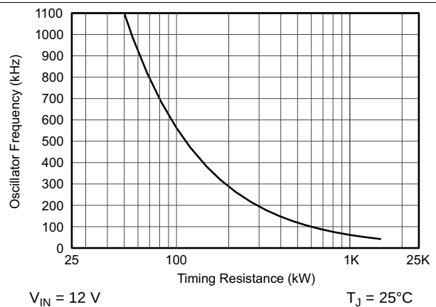
Figure 6. Frequency vs R_{\text{T/CLK}} Resistance
