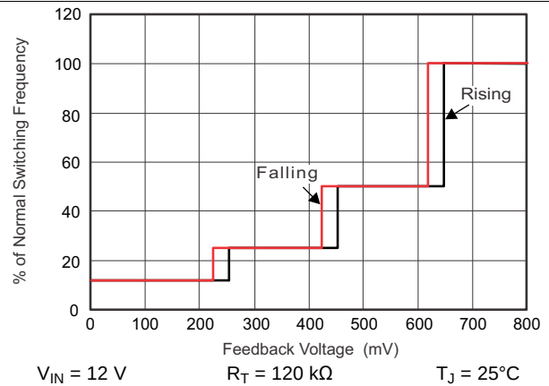
Figure 4. Frequency vs V_{\text{SENSE}} Voltage
