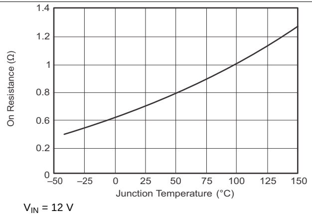
Figure 2. Low-Side r_{\text{DS(on)}} vs Temperature
