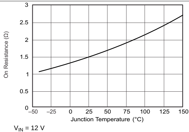
Figure 1. High-Side r_{\text{DS(on)}} vs Temperature
