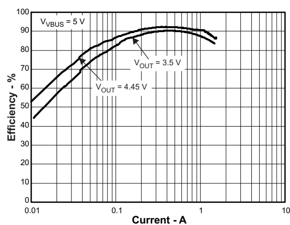
Figure 24. Charger Efficiency
