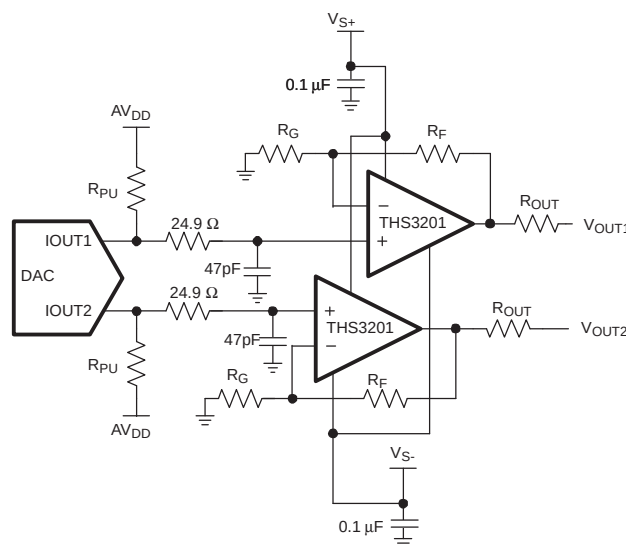
Figure 62. Differential DAC Driver Circuit
