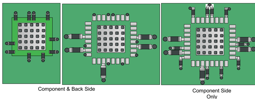
Figure 38. CDCE62002 Power Supply Bypassing
