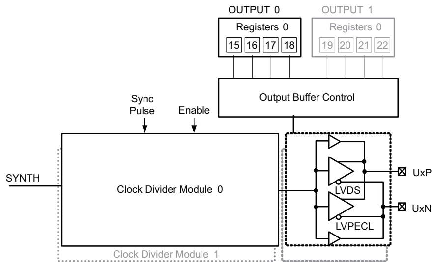
Figure 23. CDCE62002 Output Channel
