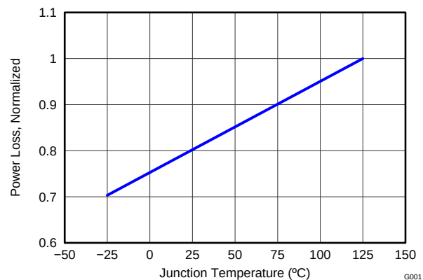
Figure 8. Power Loss vs Temperature
