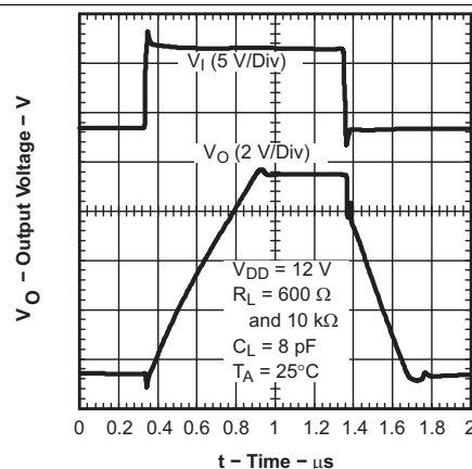
Figure 32. Large-Signal Follower Pulse Response
