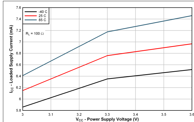
Figure 1. Loaded Supply Current vs Power Supply Voltage
