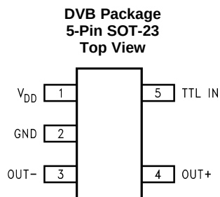
Pin Functions
