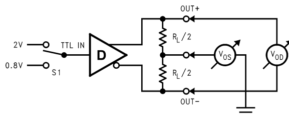
Figure 7. Differential Driver DC Test Circuit
