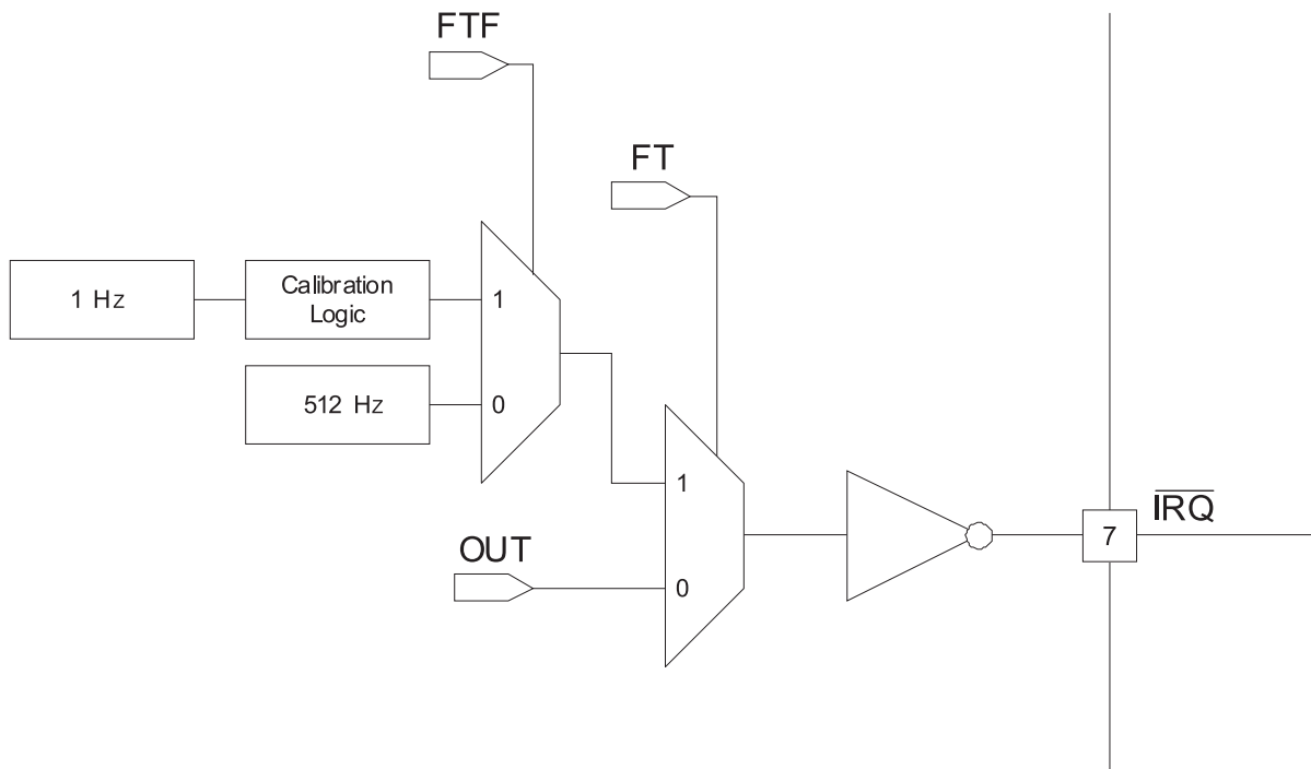
Figure 3. \overline{\text{IRQ}} Pin Functional Diagram
