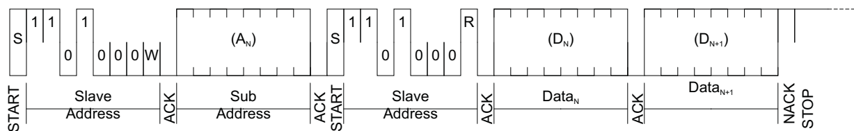
Figure 6. I²C Read Mode
