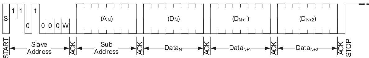
Figure 7. I²C Write Mode
