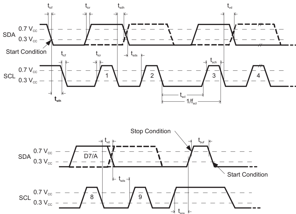
Figure 5. I²C Timing Diagram
