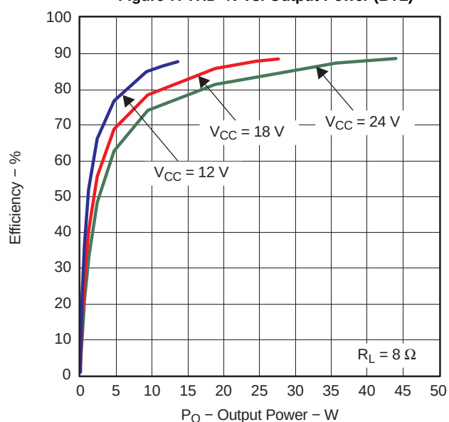
Figure 9. Efficiency Vs. Output Power (BTL)
