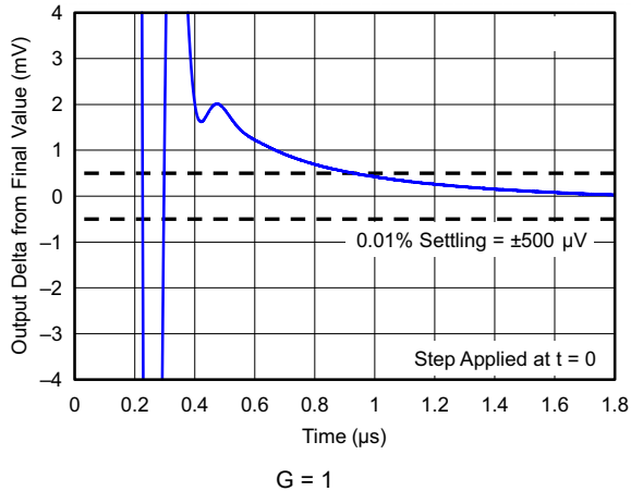
Figure 6-39. Settling Time (5-V Positive Step)
