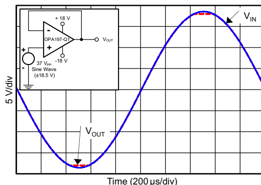
Figure 7-5. No Phase Reversal
