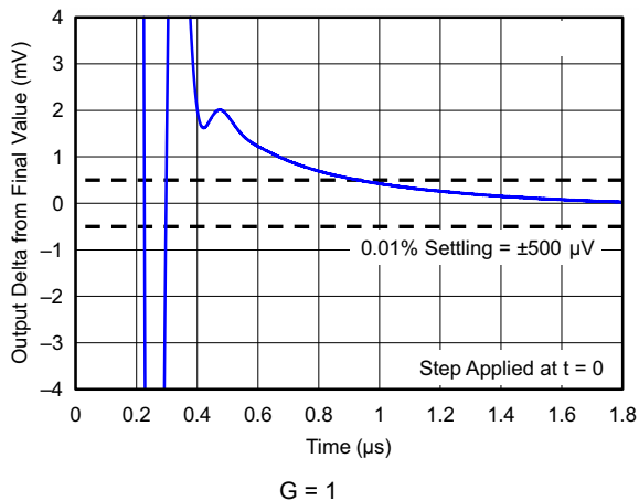
Figure 6-41. Settling Time (5-V Negative Step)
