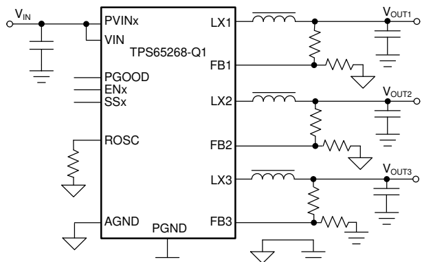
Application Schematic
