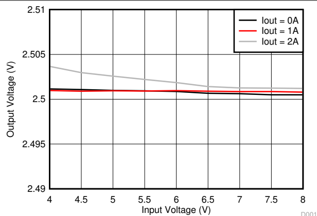
Figure 6-9. BUCK3, Line Regulation
