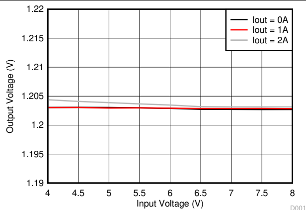
Figure 6-8. BUCK2, Line Regulation
