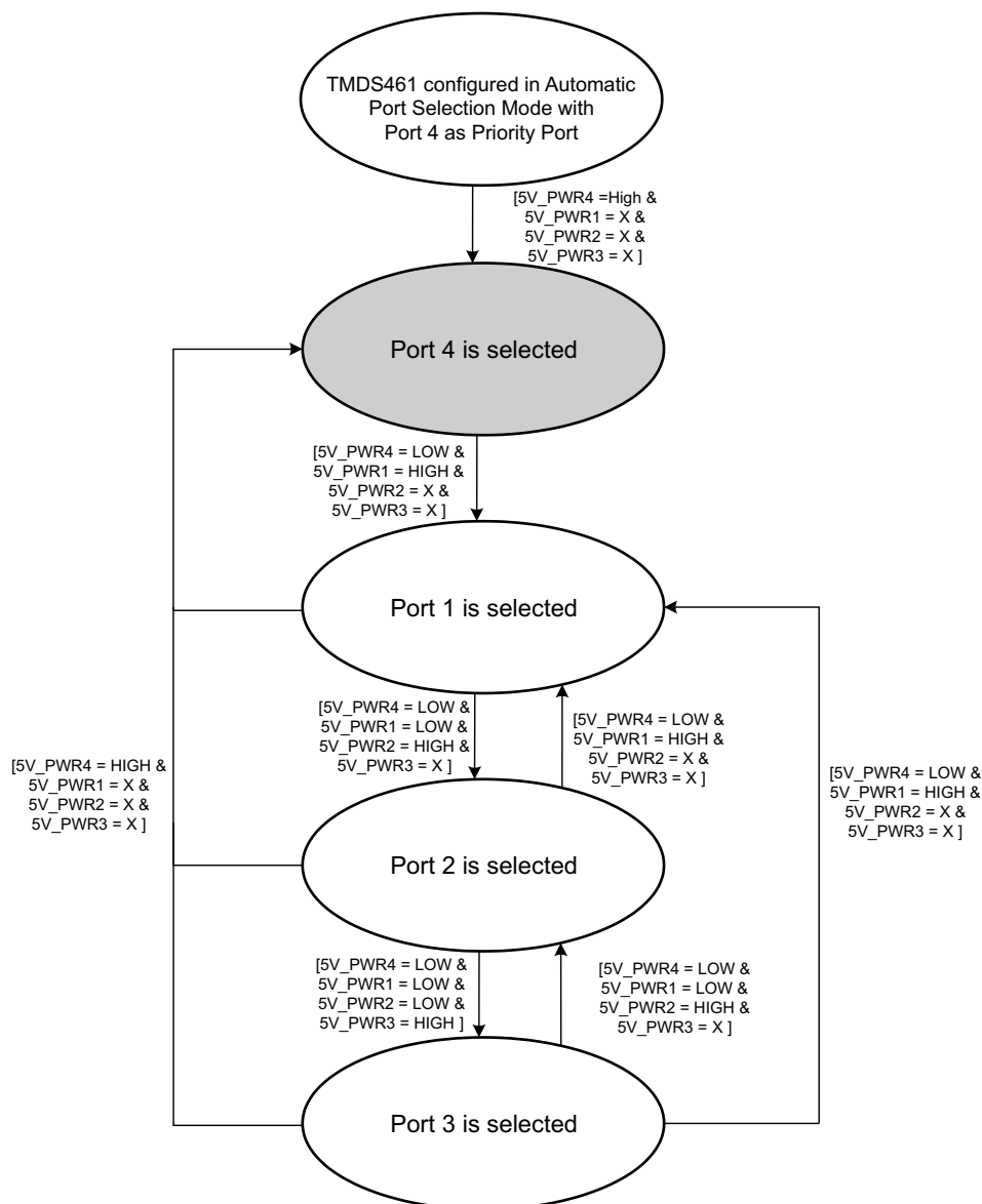
Figure 7. TMD5461 Configured in AutoSelect Mode, with Port 4 as Priority Port
