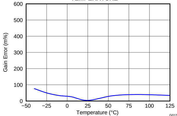
BUS MEASUREMENT INPUT GAIN ERROR vs TEMPERATURE
