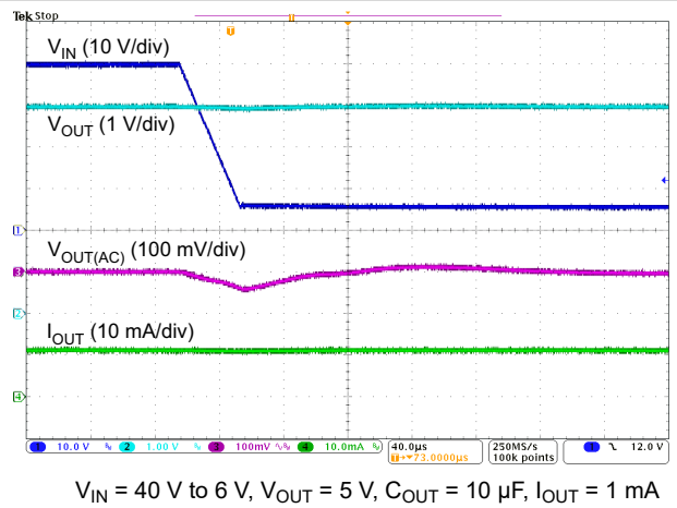
Figure 5-16. Line Transient
