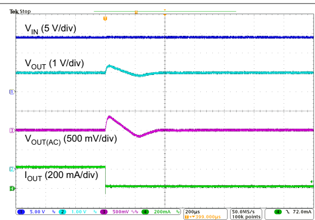
Figure 5-20. Load Transient
