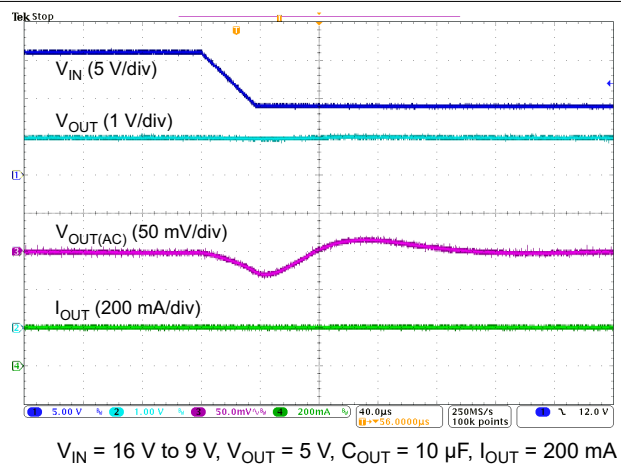
Figure 5-18. Line Transient
