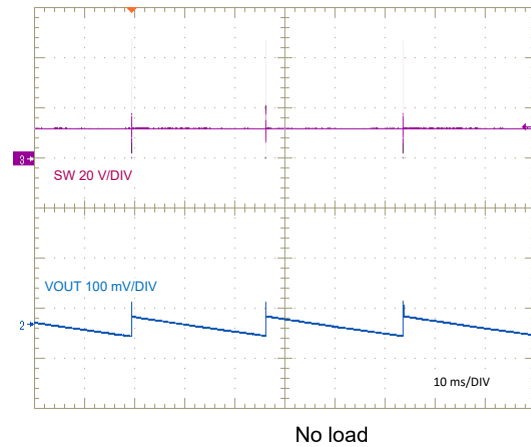
Figure 8-23. PFM Switching
