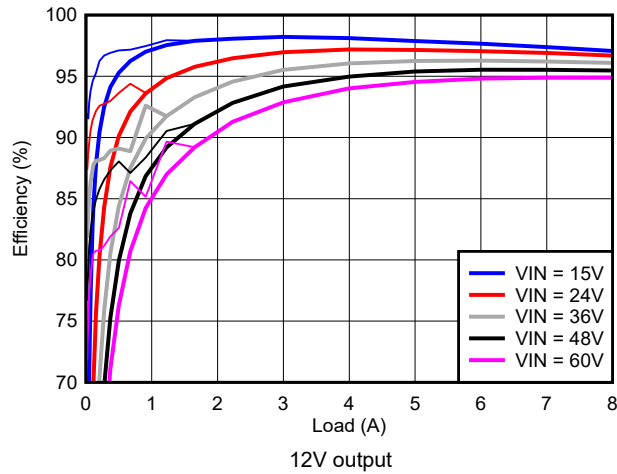
Figure 8-20. Efficiency versus I_{OUT}
