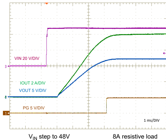
Figure 8-24. Start-Up Characteristic
