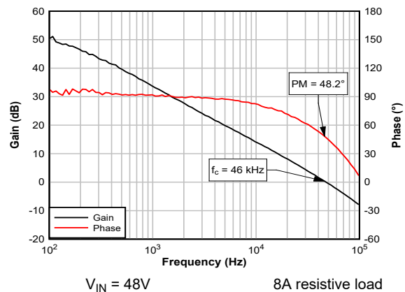
Figure 8-18. Bode Plot, 5V Output
