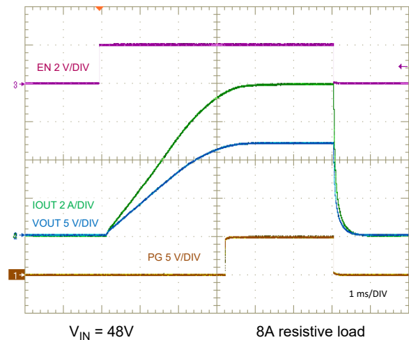
Figure 8-25. EN Start-Up Characteristic
