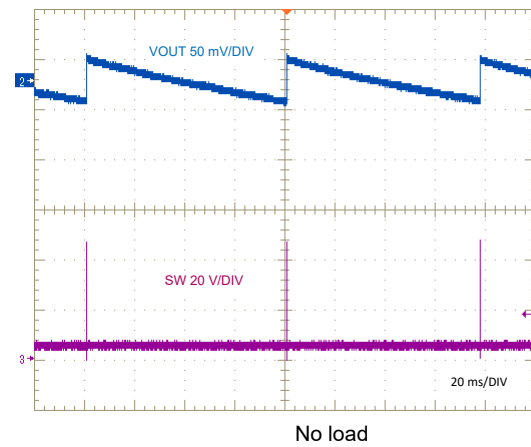
Figure 8-12. PFM Switching
