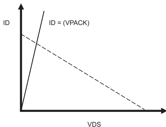
Figure 30. 0V/PCHG FET ID and VDS Characteristics
