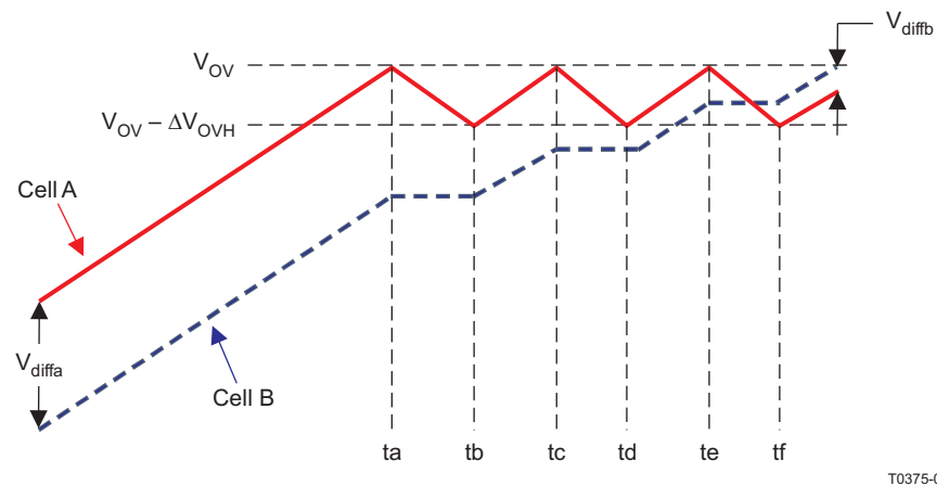
Figure 19. Cell Balancing Timing Chart (Automatic)
