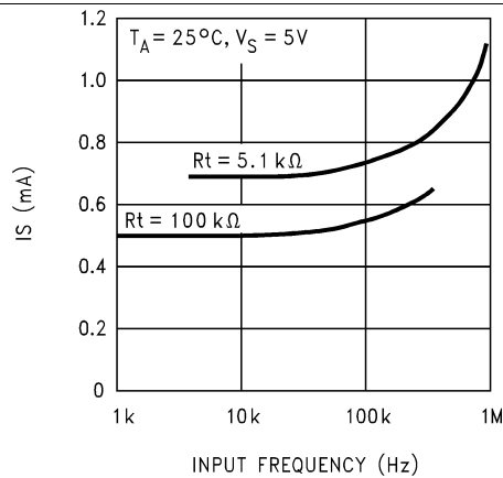
Figure 1. Supply Current vs Operating Frequency
