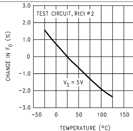
Figure 6. Frequency Drift With Temperature
