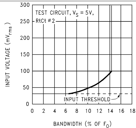
Figure 2. Bandwidth vs Input Signal Level
