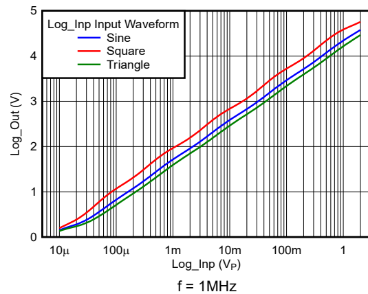
Figure 5-22. Log-Detector output for Various Input Waveforms
