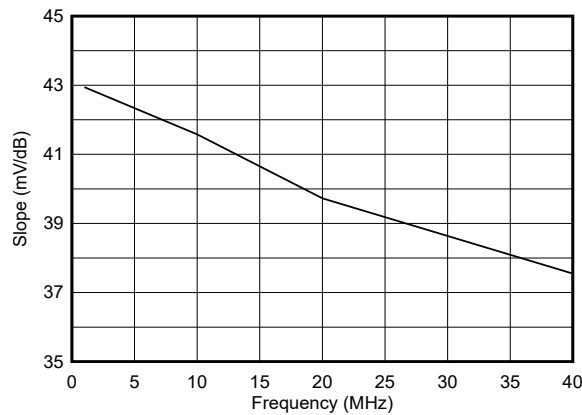
Figure 5-9. Log-Detector Slope Variation with Input Signal Frequency
