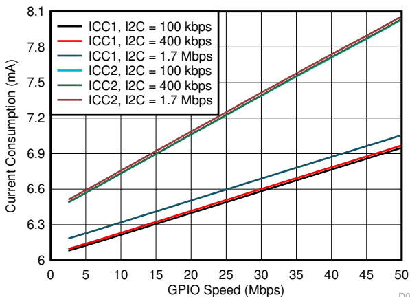
Figure 6-21. ISO1642: ICC vs GPIO Speed at 3.3V
