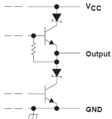
Figure 6-2. Typical of All Driver Outputs
