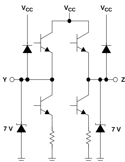
OUTPUT LVDS20
