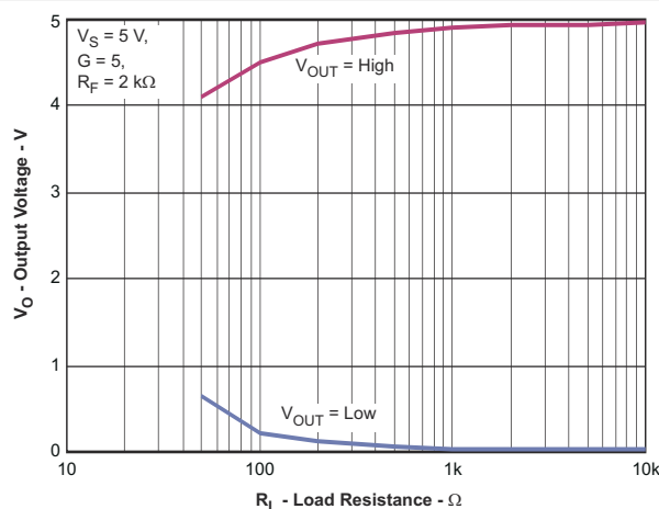
Figure 7-37. Output Voltage Swing vs Load Resistance
