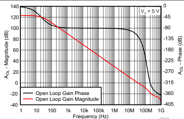
Figure 7-43. Open-Loop Gain vs Frequency
