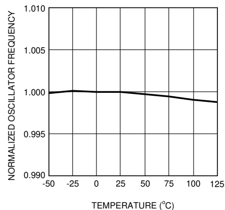
Figure 5-2. Oscillator Frequency vs Temperature F_{OSC} = 200\text{kHz}
