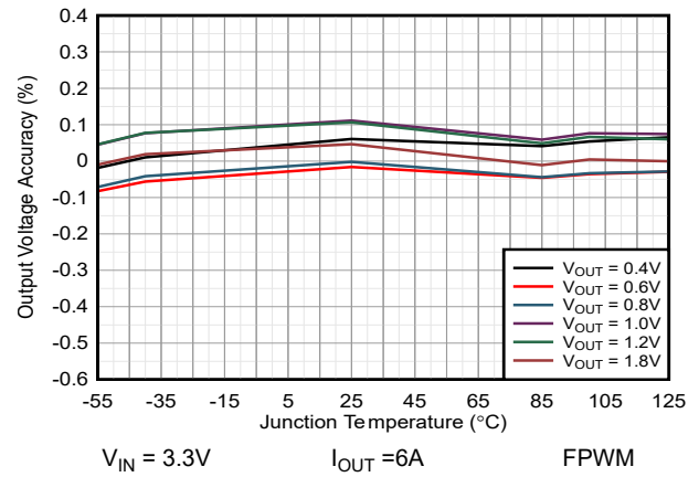
Figure 9-17. Vout Accuracy vs Temperature TPSM8287A12BAM
