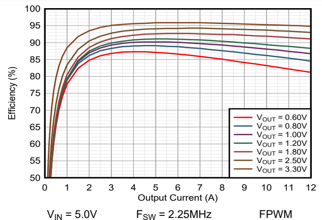
Figure 9-7. Efficiency TPSM8287A12BBM
