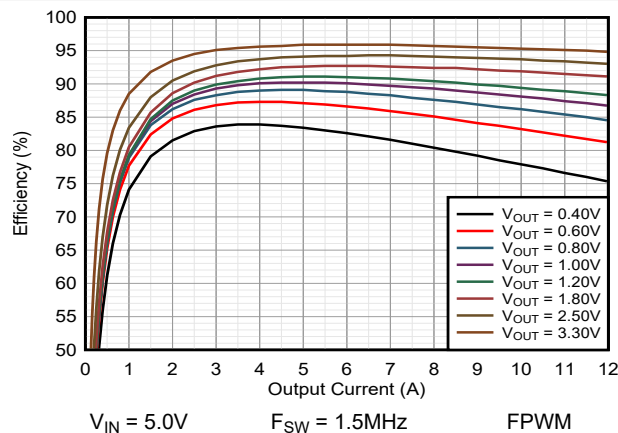
Figure 9-6. Efficiency TPSM8287A12BAM
