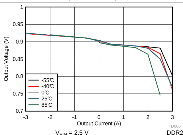
Figure 7. Load Regulation
