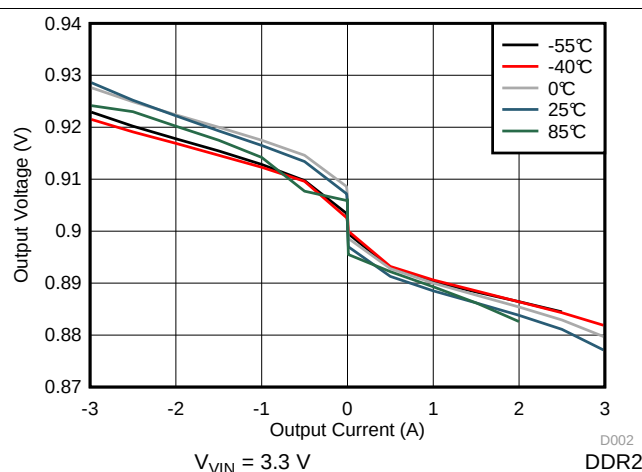
Figure 3. Load Regulation
