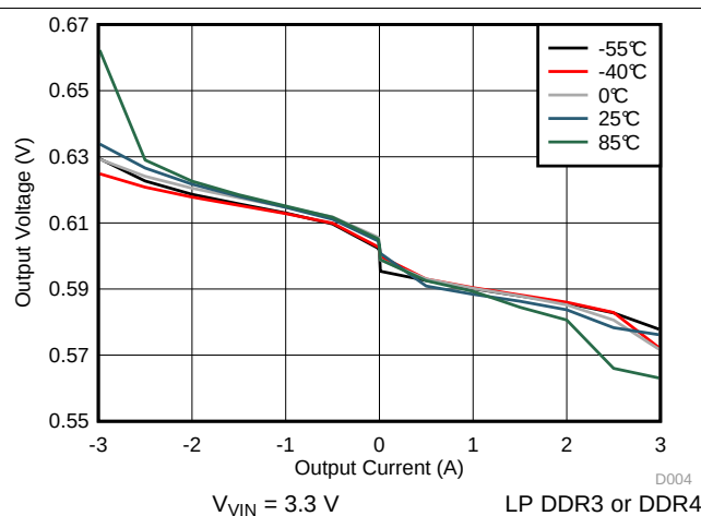
Figure 5. Load Regulation
