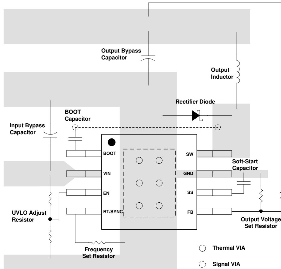
Figure 7-10. Layout Example
