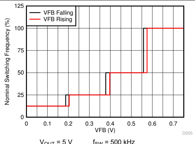
Figure 5-6. Frequency vs V_{FB}
