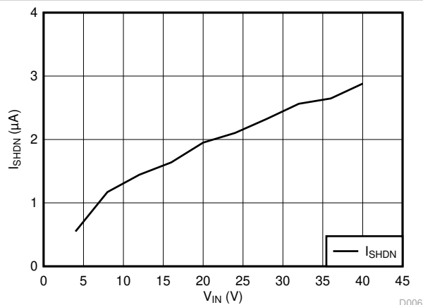
Figure 5-11. Shutdown Current
