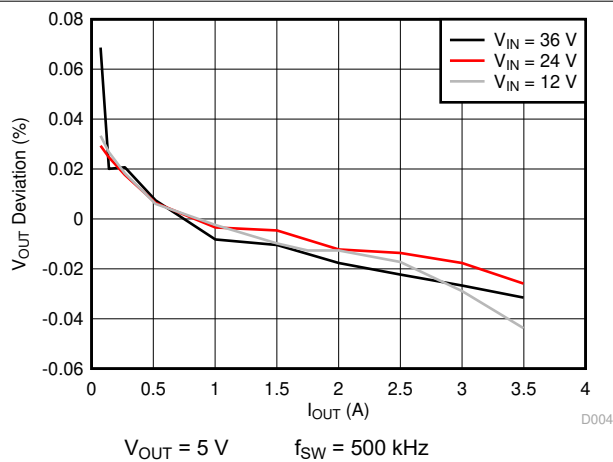
Figure 5-5. Load Regulation
