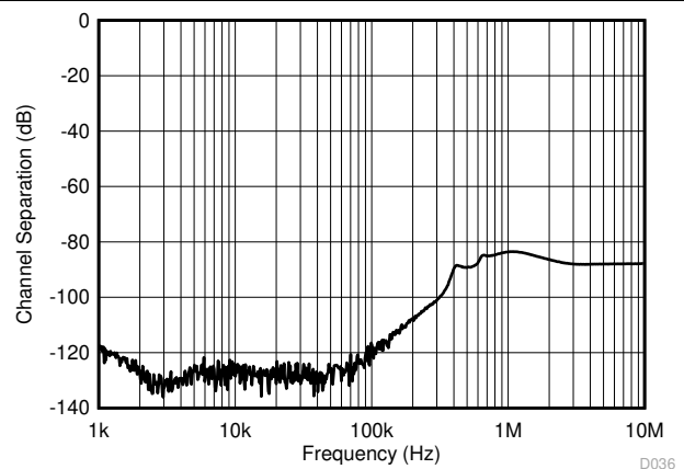
Figure 6-29. Channel Separation
