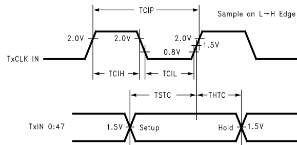
Figure 5. DS90CR483A (Transmitter) Setup/Hold and High/Low Times
