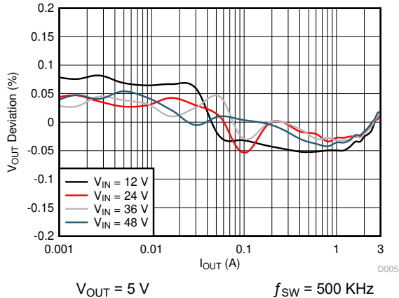
Figure 7-5. Load Regulation
