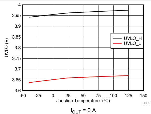
Figure 7-10. UVLO Threshold
