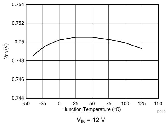
Figure 7-8. Voltage Reference vs Junction Temperature
